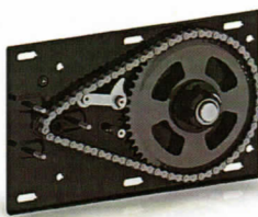
TS 300B cod.1780013 Motor bracket transmission gear ratio 1:6 without cover.
